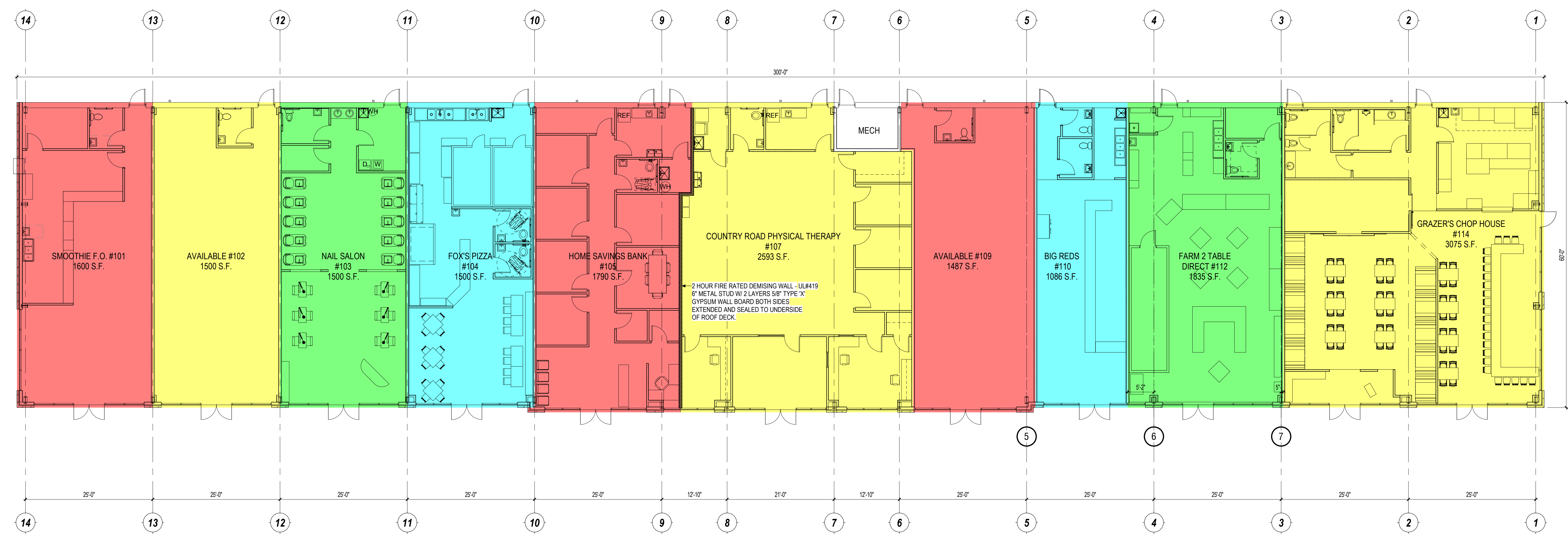
TENANT PLAN SCALE: 1" = 10'-0" SHEET TP-1
